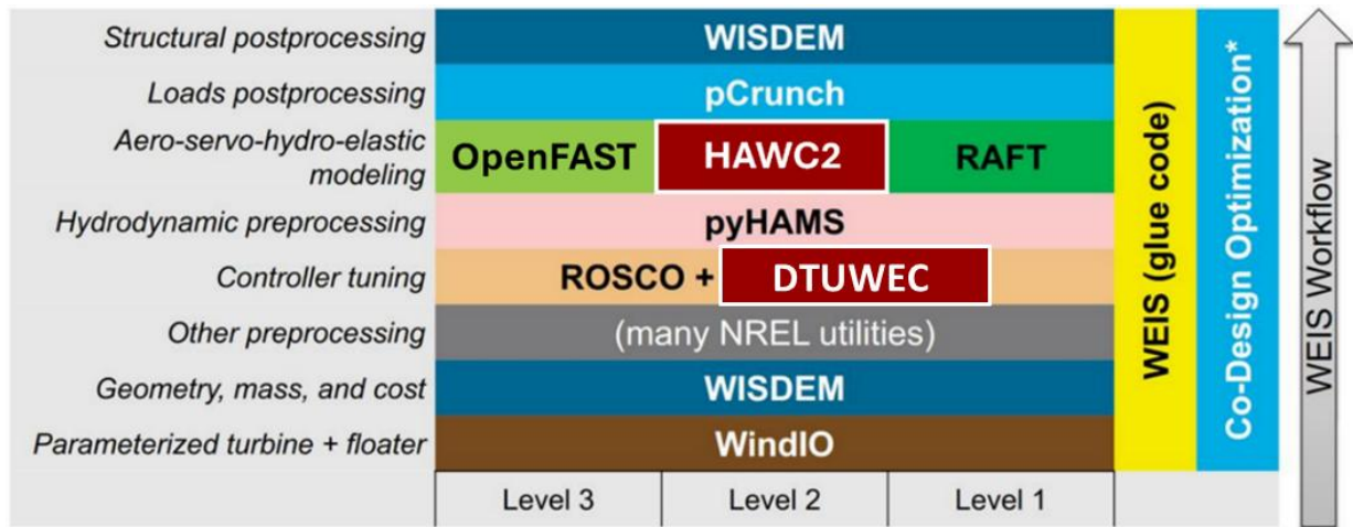
Figure 3 – HAWC2 in the WEIS Framework, taken from [6] and modified.
