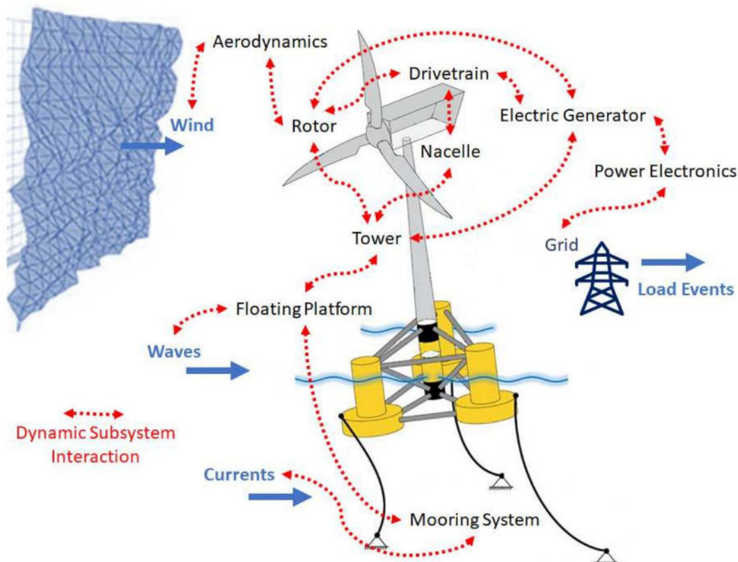
Figure 1 – Sub-systems of a FOWT and environmental excitation. Figure taken from [3].
