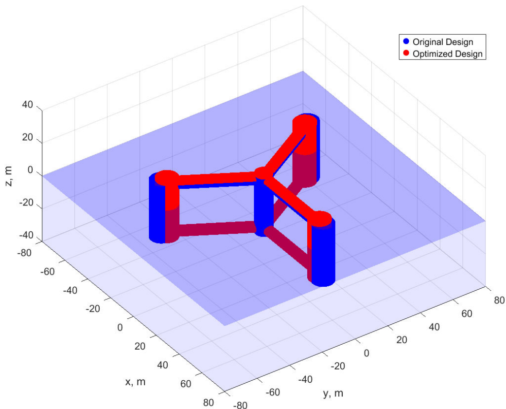
Figure 9 – Comparing the geometries of the original and optimized VoltturnUS-S platform.
