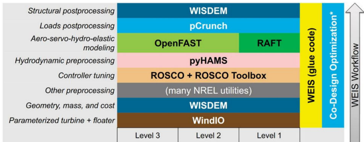
Figure 2 – Components that are integrated in WEIS, taken from [6].
