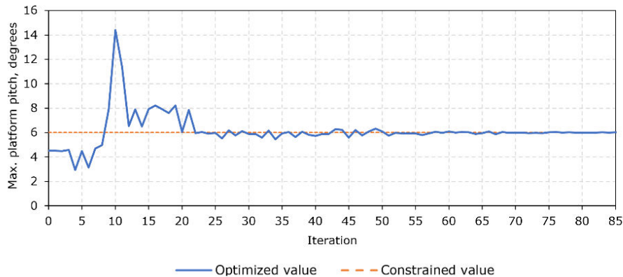
Figure 8 - Iterative changes to the maximum platform pitch angle constraint during the optimization.
