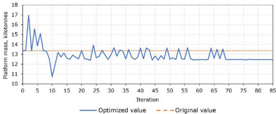
Figure 6 – Iterative changes to the platform mass during the optimization.
