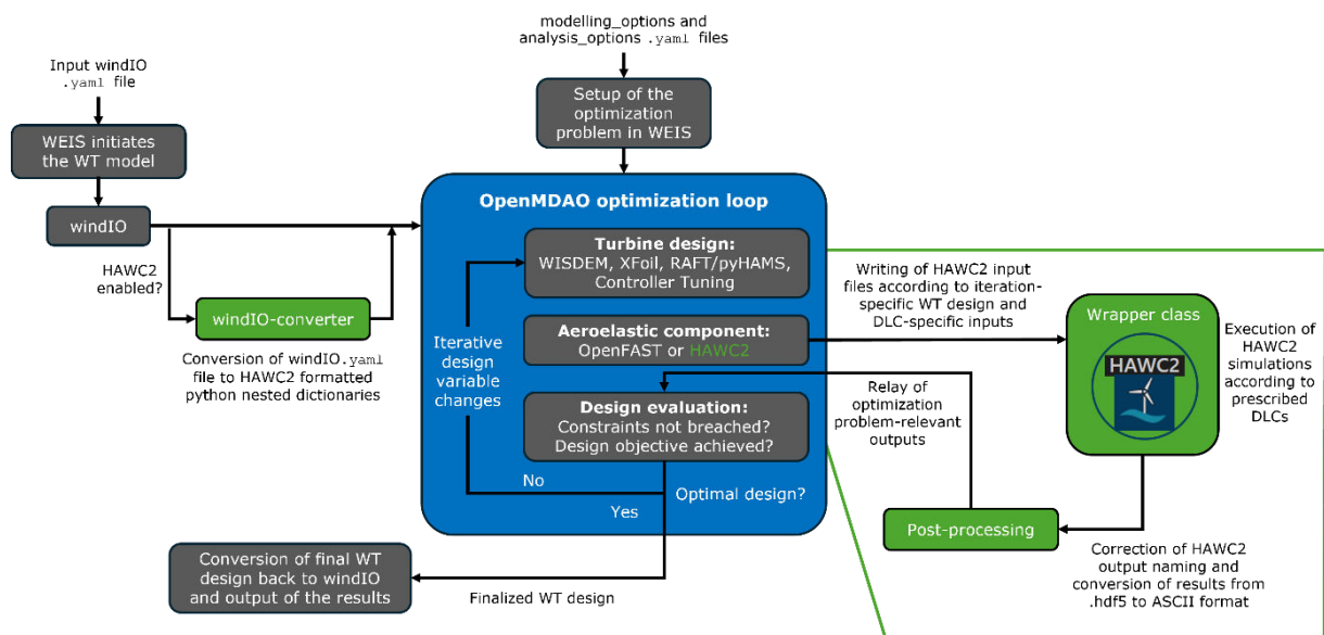
Figure 4 - Flowchart illustrating the WEIS optimization framework and where the newly implemented HAWC2 solver lies within it. Grey boxes represent existing WEIS functionality and green boxes/text represent the additions made to achieve the HAWC2 integration.
