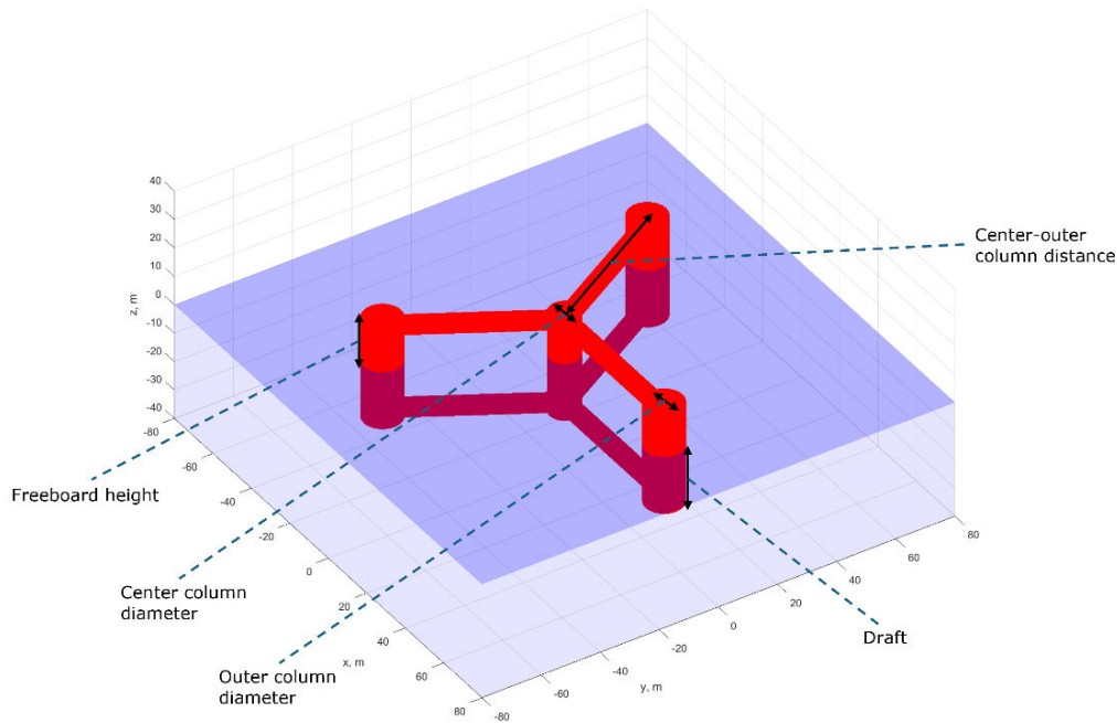
Figure 5 – Properties of the VoltturnUS-S platform geometry set as design variables (excluding the outer column wall thickness).
