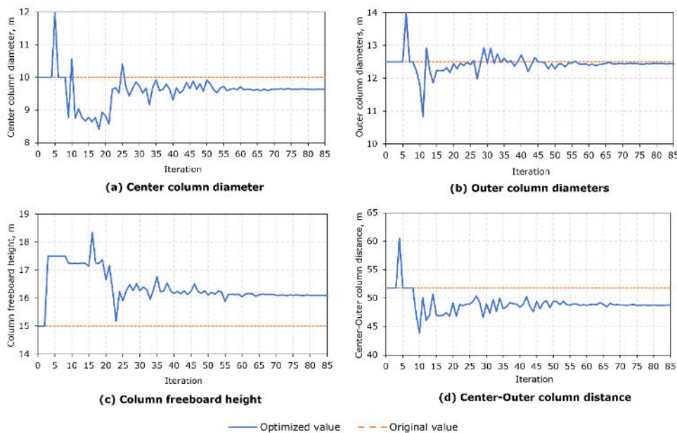
Figure 7 - Iterative changes to the design variables during the optimization.
