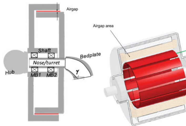
Figure 2 Illustration of a conventional radial flux direct drive generator as part of the wind power nacelle, highlighting the airgap area in red.
