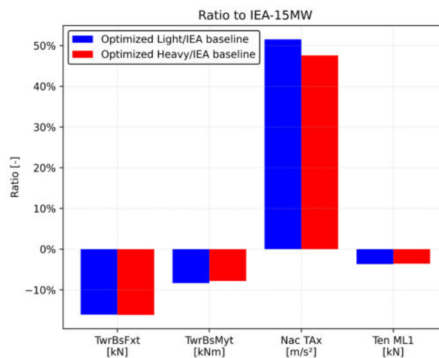
Figure 18 In red, the ratio (expressed as a relative percentage) of mean extreme load values for the optimized system with the heavy Hagnesia generator to that of the baseline IEA-15MW turbine. In blue, the same ratio for the optimized system with the light Hagnesia generator, relative to the baseline.
