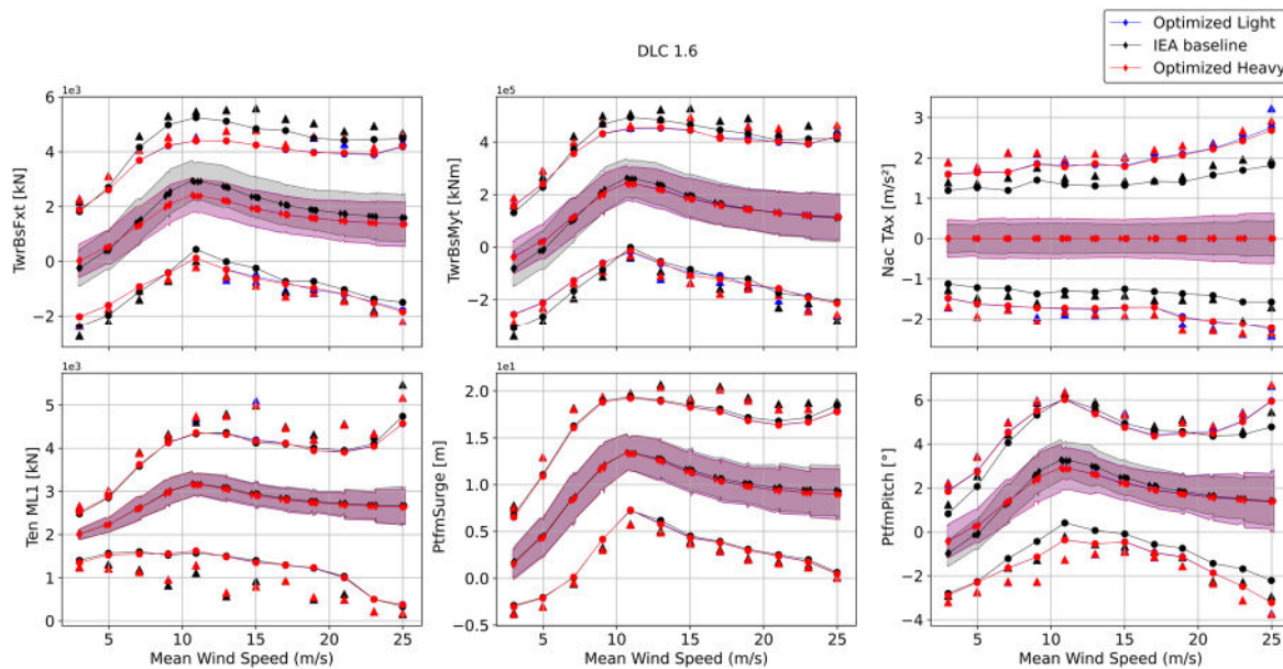
Figure 16 Comparison of tower base force in x-direction (TwrBsFxt), tower base bending moment in y-direction (TwrBsMyt), nacelle fore-aft acceleration (Nac TAX), upwind mooring line tension (Ten ML1) and platform displacement in x-direction (PtfmSurge) along with platform pitch (PtfmPitch) mean value, standard deviation (shaded), maxima and minima per wind speed recorded in DLC 1.6. Triangles refer to DLC 1.6 maxima values and dots are referred to DLC1.6 means of maxima.
