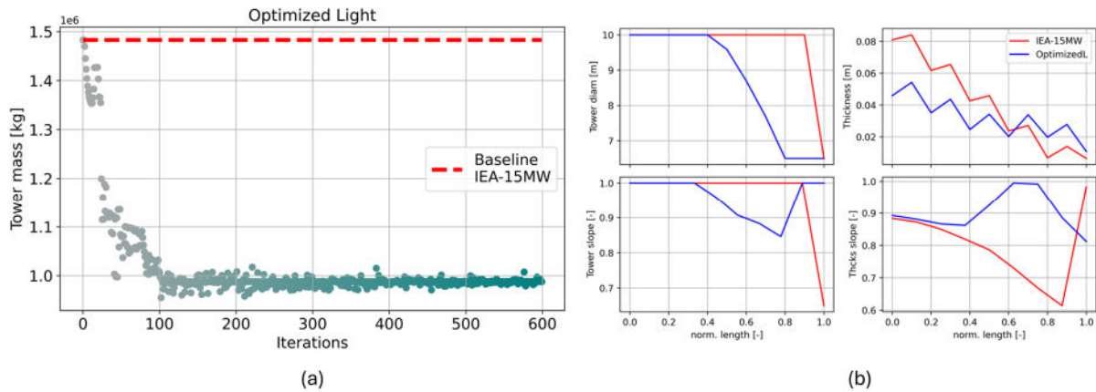
Figure 14 Lighter Hagnesia Generator tower optimization, (a) shows merit figure (tower mass) convergence trend compared with base line IEA tower mass. Comparison between IEA-15MW RWT geometry and optimized tower is shown in (b).
