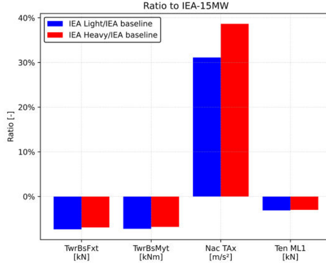
Figure 12 In red, the ratio (expressed as a relative percentage) of the mean extreme load values for the IEA-15MW turbine with the heavy Hagnesia generator to that of the baseline IEA-15MW turbine. In blue, the same ratio for the IEA-15MW turbine with the light Hagnesia generator, relative to the baseline model.
