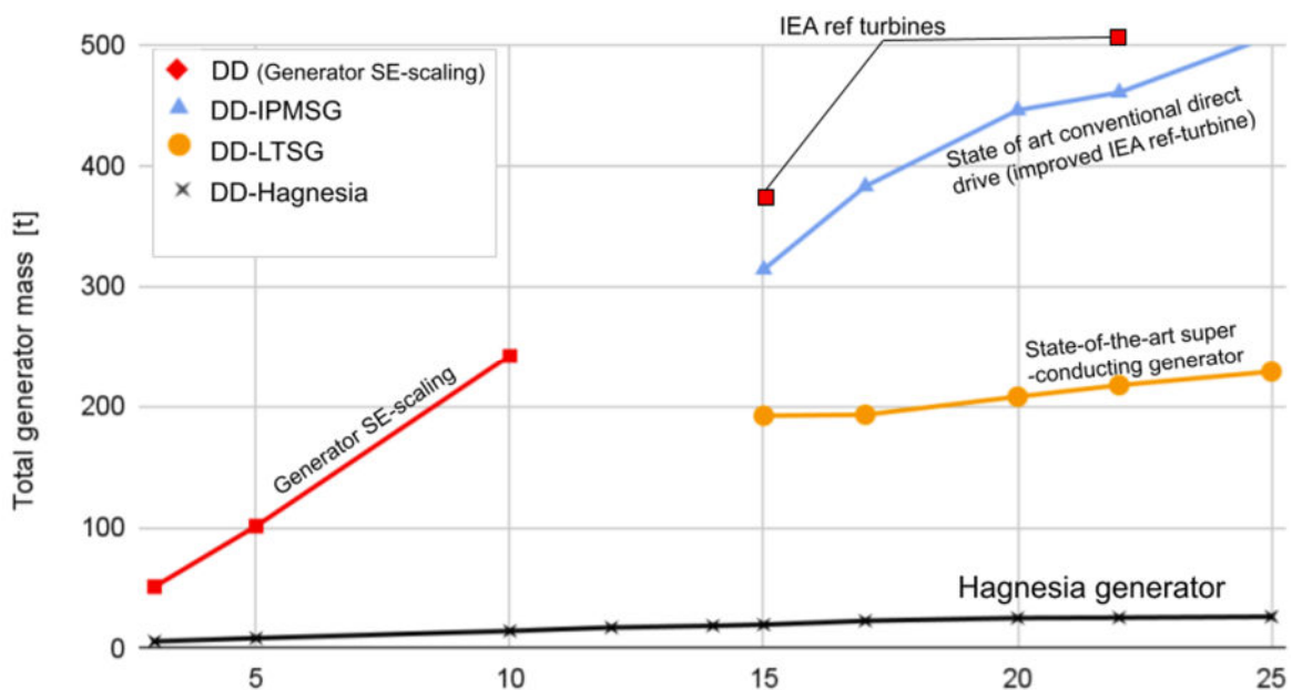
Figure 8 Weight comparison of the Hagnesia direct drive generator to other state-of-the-art generator technologies, as further described in text.
