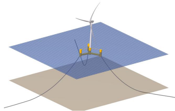
Figure 6– IEA22MM on UMaine VoltturnUS-S platform, rendered in the QBlade GUI
